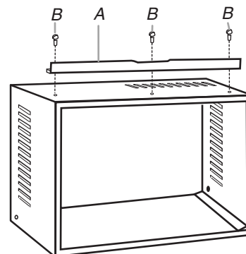
A. Top channel B. #10 x \frac{3}{8} " washer-head Phillips screws (3)
