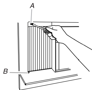
A. #10 x \frac{3}{4} " round-head screw B. Hole for #10 x \frac{3}{4} " round-head screw
