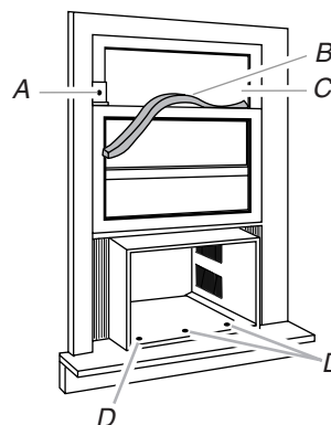
A. Window lock bracket B. Foam window sash seal C. Upper window glass D. #10 x \frac{1}{2} " pan-head Phillips screws (3)
